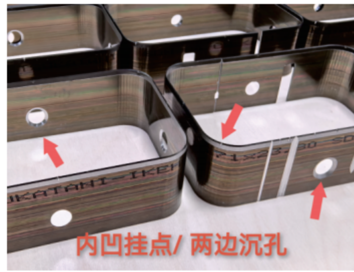
内凹挂点、两边沉孔 Inner Nick,Countersunk Hole
